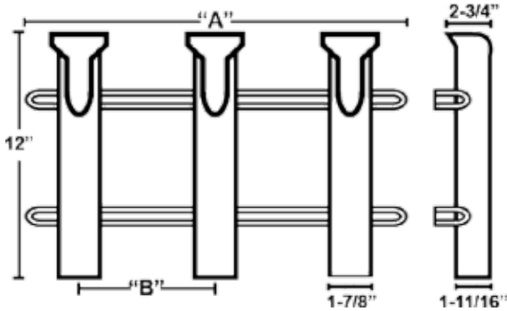
Light rod holder with closer rod holder spacing
