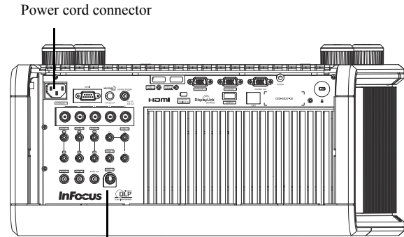
Connector panel
