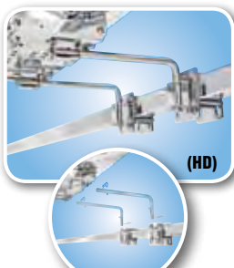
Extended "Dual" Side, Bulkhead or Square/Flat Rail Mount Fits up to 2-1/4" (57 mm) sq. rail T10-640
