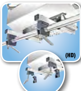
"Dual" Extended Horizontal Round Rail Mount T10-680 Standard Rails 1" (25.5 mm) T10-685 Oversize Rails 1-1/4" (32 mm) T10-690 Large Rails 1-1/2" (38 mm)
