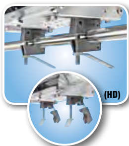
"Dual" Horizontal Round Rail Mount T10-580 Standard Rails 7/8" or 1" (22 mm or 25.5 mm) T10-585 Oversize Rails 1-1/8" or 1-1/4" (28.5 mm or 32 mm) T10-590 Large Rails 1-1/2" (38 mm)
