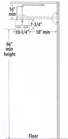
0° installation to combustible (side view)
