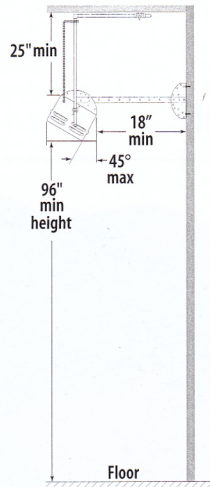
45° installation to combustible (side view)
