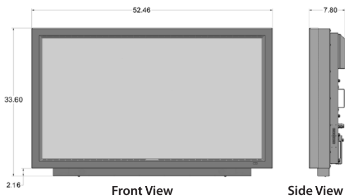
Dimensions with detachable speaker module. All measurements are in inches
