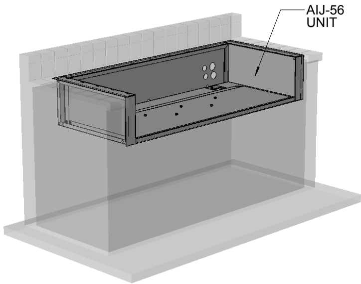
AIJ-56 TYPICAL INSTALLATION
