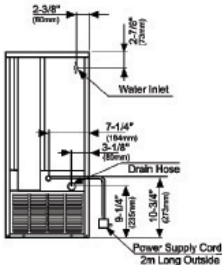
BACK DIMENSIONS
