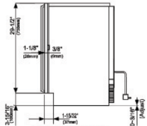
SIDE DIMENSIONS
