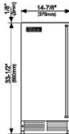
FRONT DIMENSIONS
