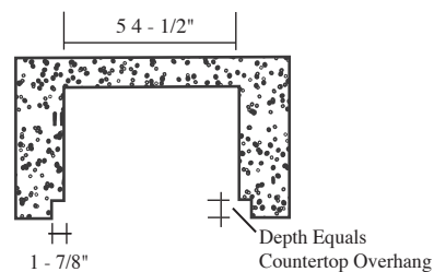
COUNTERTOP DETAIL
