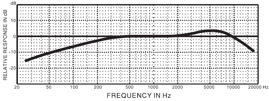
QL5 FREQUENCY RESPONSE
