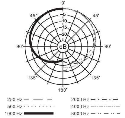
QL5 POLAR PATTERN
