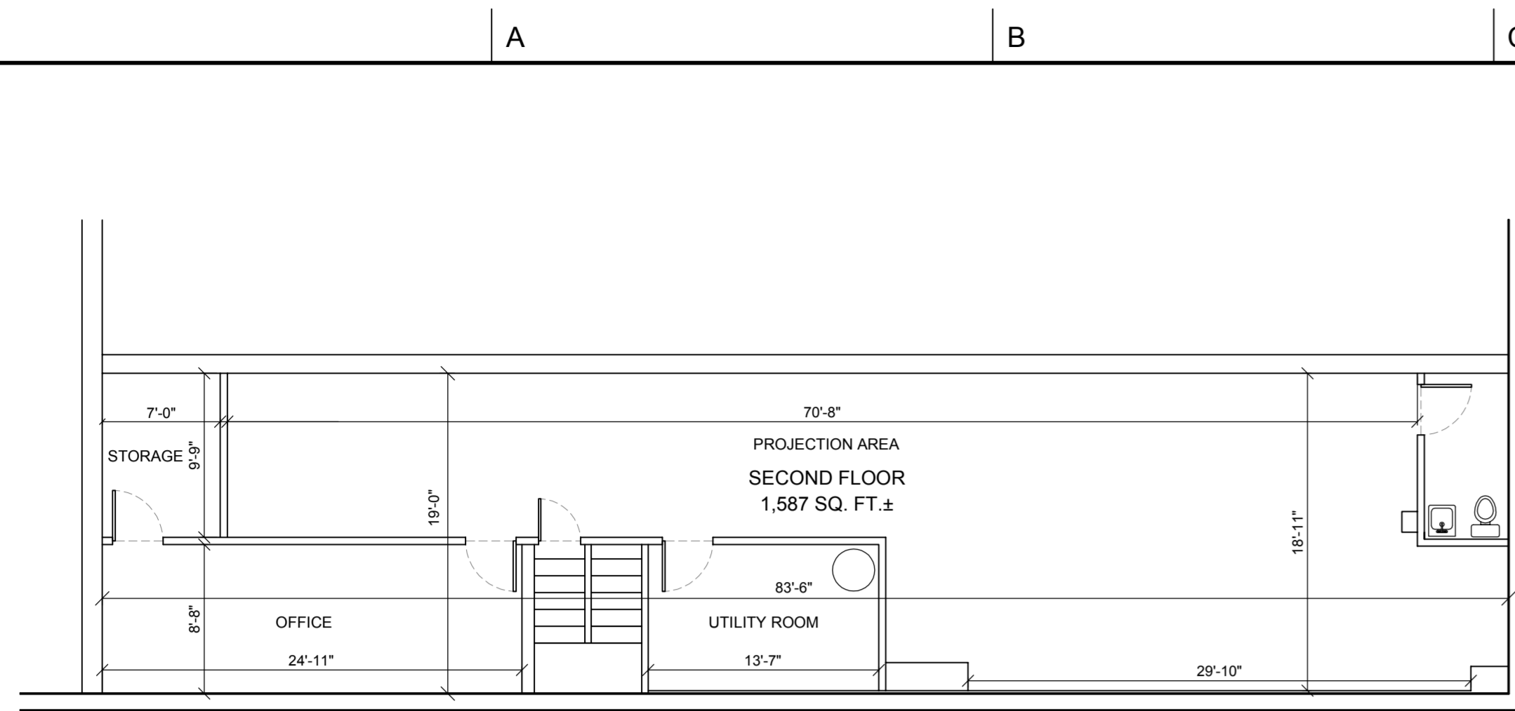
SECOND FLOOR - PROJECTION AREA SCALE: 1/8"=1'-0"
