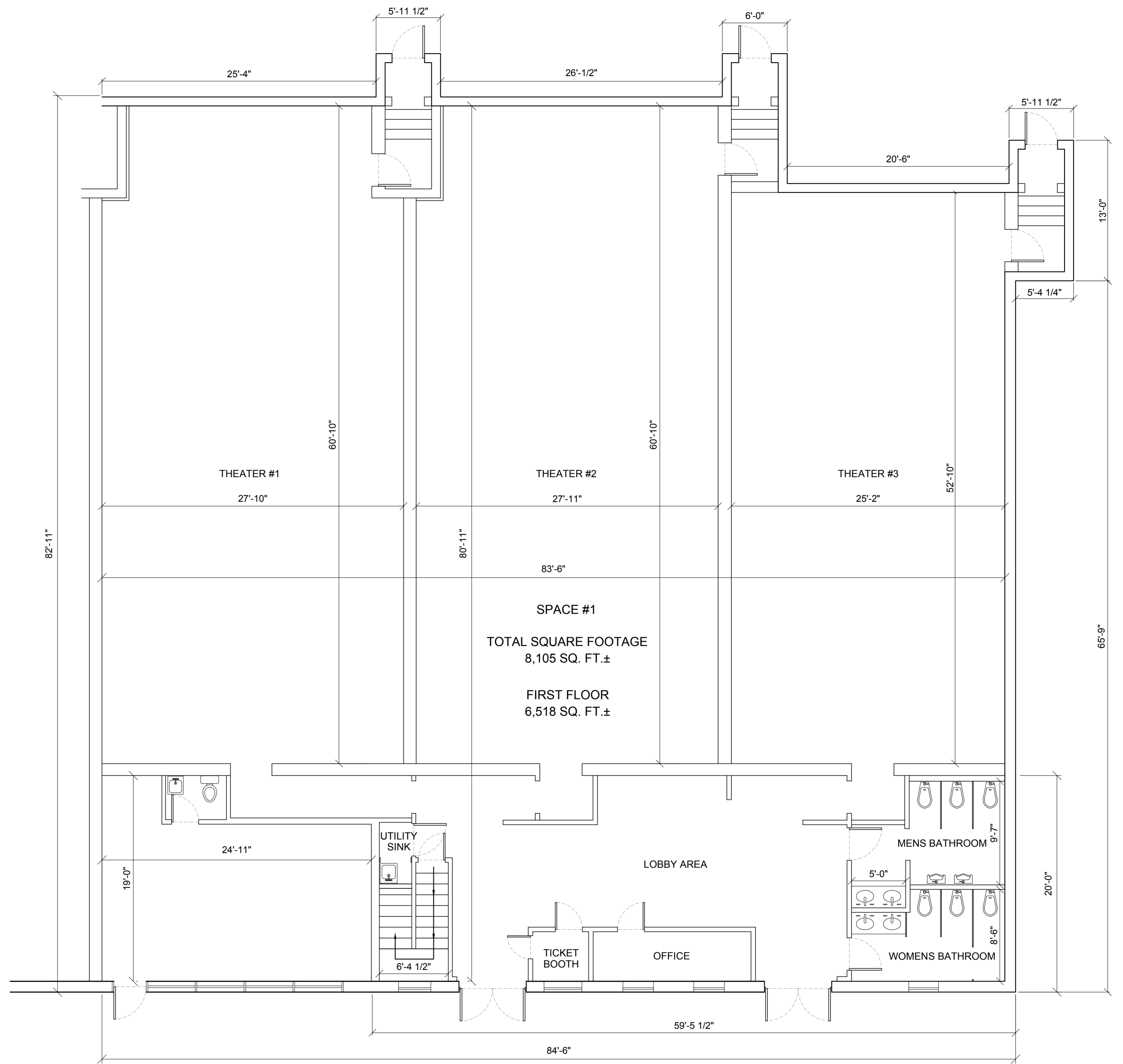
FIRST FLOOR - CINEMA AREA
