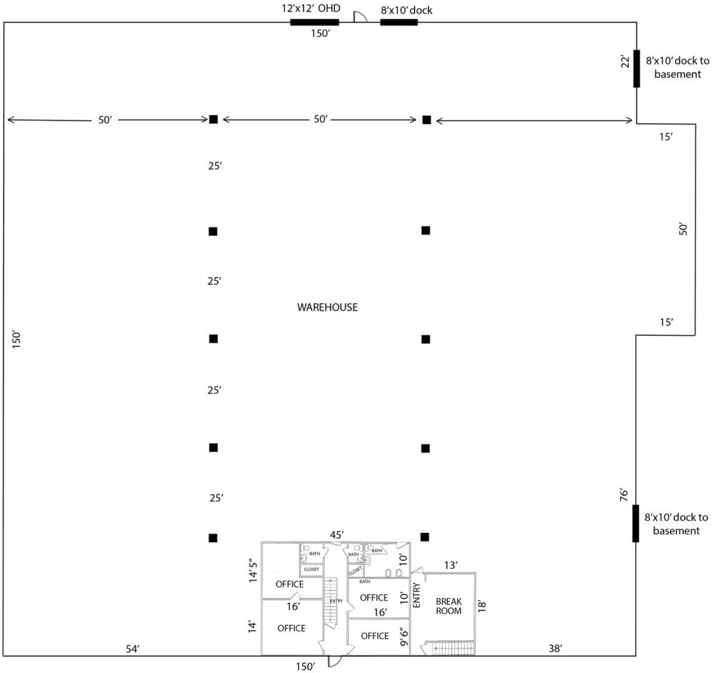
FLOOR PLAN 864 WEST STREET, WATERTOWN WI
