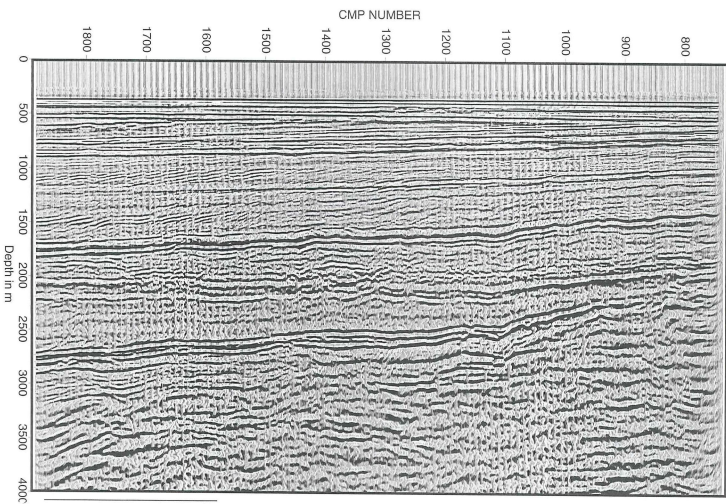
Figure 4.20 Post stack migration of the Radon stack using the velocity model estimated with curvature parameters.
