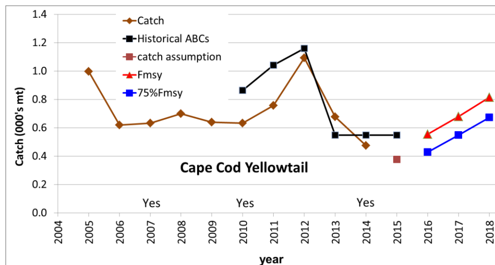
Figure 9- Catch performance for Cape Cod/Gulf of Maine yellowtail flounder including: catches from CY 2005- CY 2014, historical ABCs since FY 2010, CY 2015 “bridge year” catch assumption, and projections for FY 2016- FY 2018 at F_{MSY} and 75\%F_{MSY} . Overfishing status in the terminal year of the assessment indicated on the x-axis (Yes = overfishing, No= not overfishing, and unknown = unknown overfishing status).
