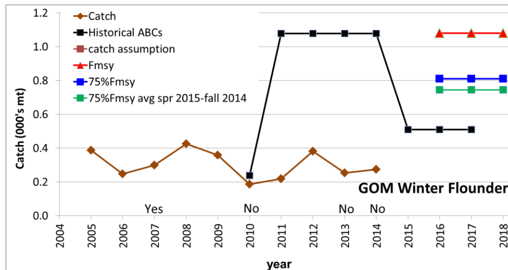
Figure 13- Catch performance for Gulf of Maine winter flounder including: catches from CY 2005- CY 2014, historical ABCs since FY 2010, CY 2015 “bridge year” catch assumption, and projections for FY 2016- FY 2018 at F_{MSY} , 75\%F_{MSY} and a sensitivity that averages 2015 spring and 2014 fall biomass. Overfishing status in the terminal year of the assessment indicated on the x-axis (Yes = overfishing, No= not overfishing, and unknown = unknown overfishing status).
