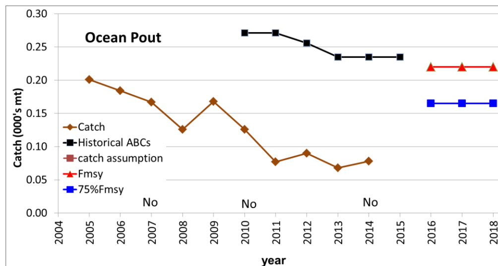
Figure 20- Catch performance for ocean pout including: catches from CY 2005- CY 2014, historical ABCs since FY 2010, CY 2015 “bridge year” catch assumption, and projections for FY 2016- FY 2018 at F_{MSY} and 75\%F_{MSY} . Overfishing status in the terminal year of the assessment indicated on the x-axis (Yes = overfishing, No= not overfishing, and unknown = unknown overfishing status).
