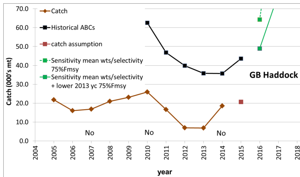
Figure 5- Detail for FY 2010 – FY 2014 Georges Bank haddock catch performance. Projections for FY 2016- FY 2018 provided as a sensitivity of likely density dependent growth and a sensitivity of likely density dependent growth with reductions in the estimated 2013 year class strength. Overfishing status in the terminal year of the assessment indicated on the x-axis (Yes = overfishing, No= not overfishing, and unknown = unknown overfishing status).
