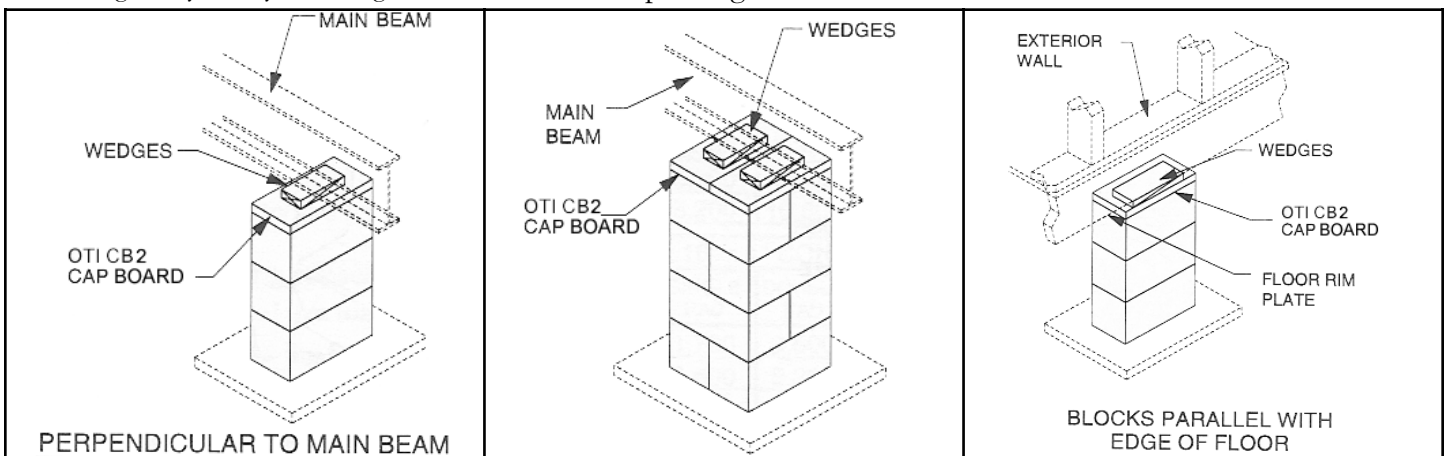
SINGLE STACK PIER
