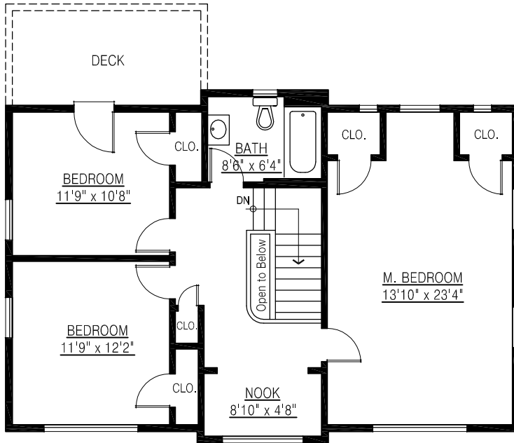
UPPER FLOOR PLAN FLOOR AREA: 930 sq.ft.
