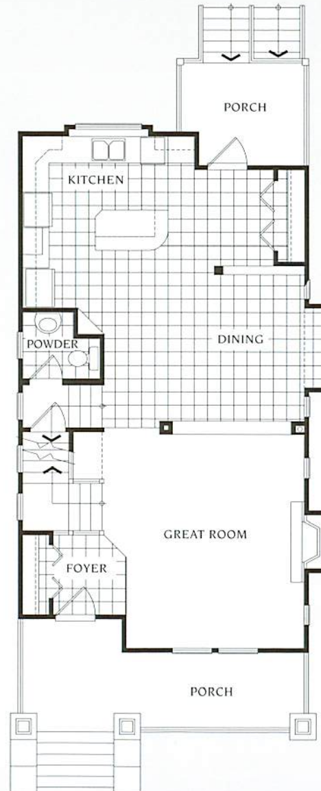
Main Floor
