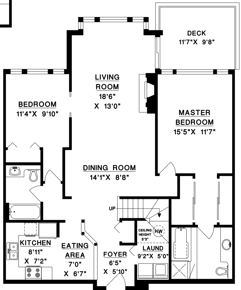
MAIN LEVEL
