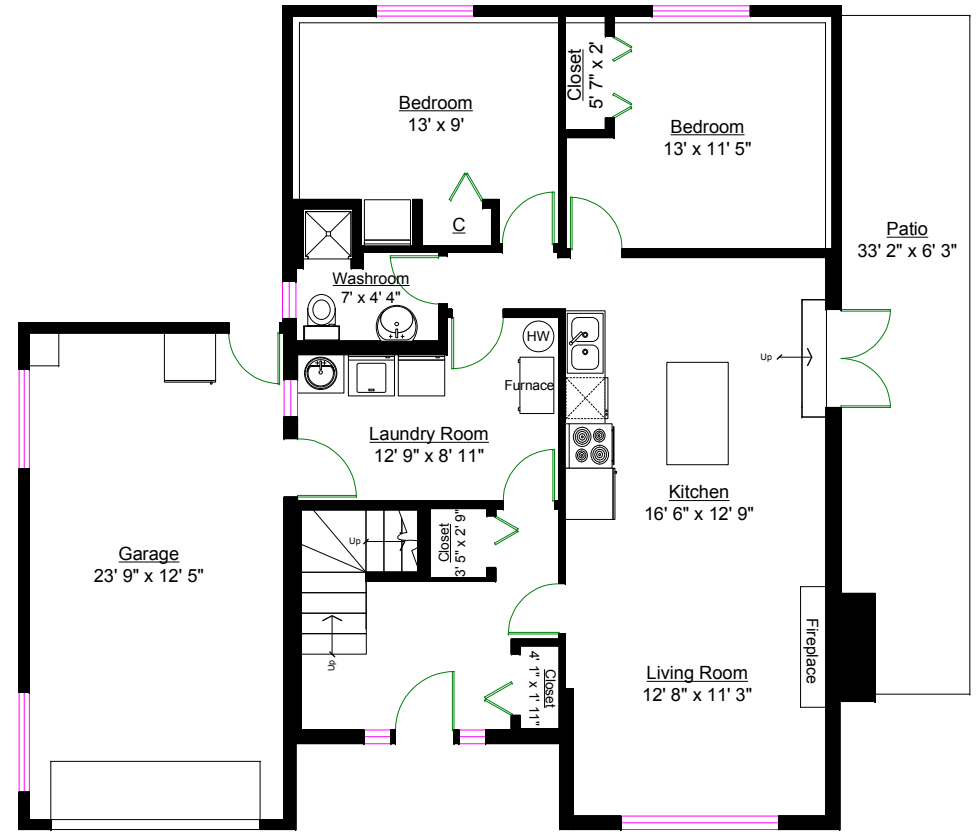
LOWER LEVEL
