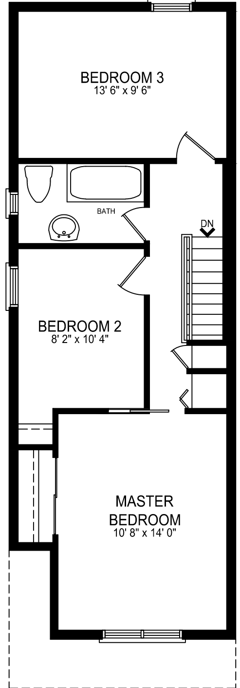
SECOND FLOOR PLAN APPROX. 588 SQ.FT.
