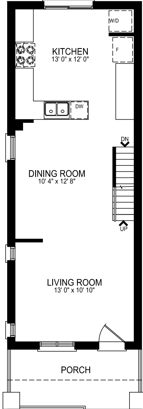
GROUND FLOOR PLAN APPROX. 555 SQ.FT.
