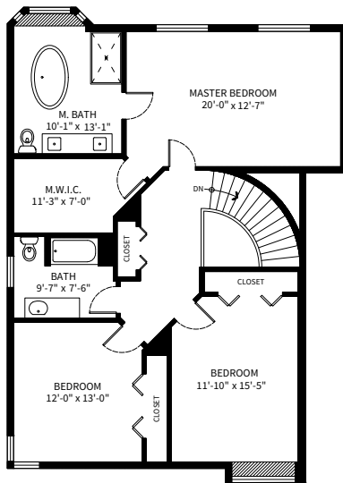
UPPER FLOOR PLAN Ceiling Height: 8'-0"
