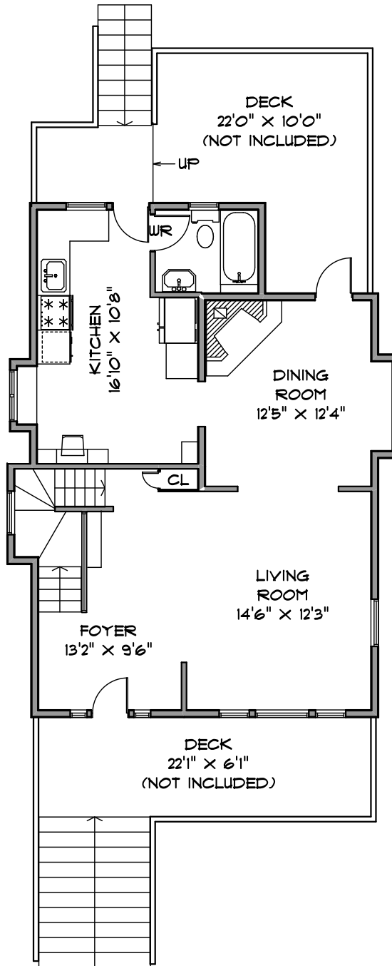
MAIN LEVEL T12 612 SQ. FT.
