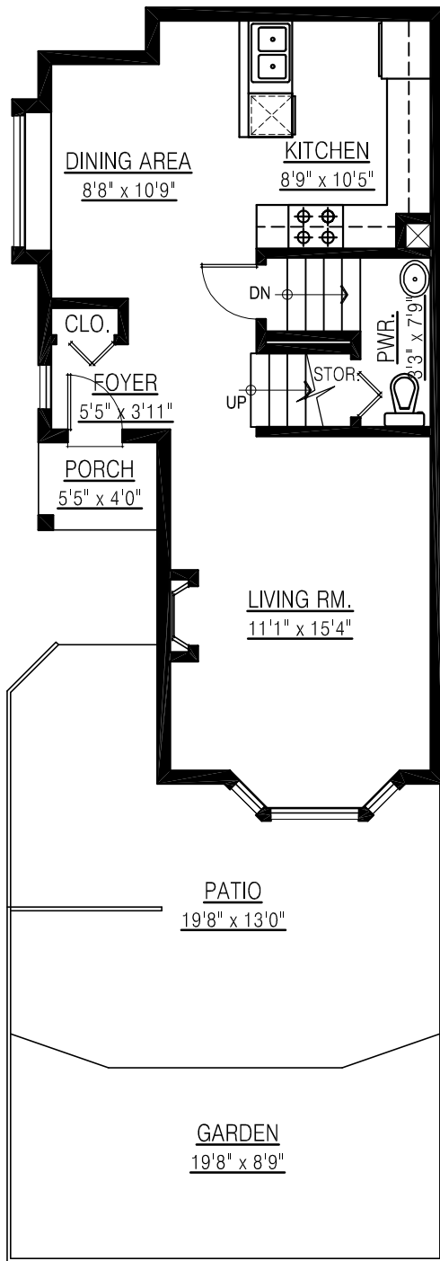
MAIN FLOOR PLAN FLOOR AREA: 583 sq.ft.
