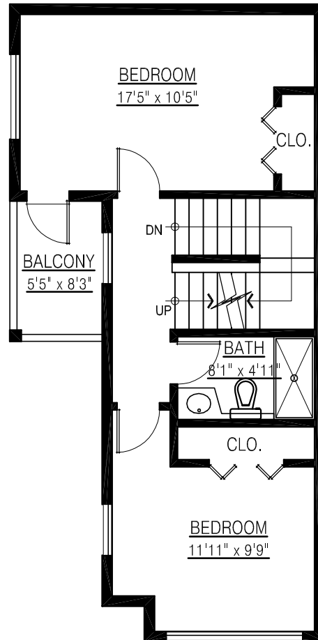
UPPER FLOOR PLAN FLOOR AREA: 550 sq.ft.
