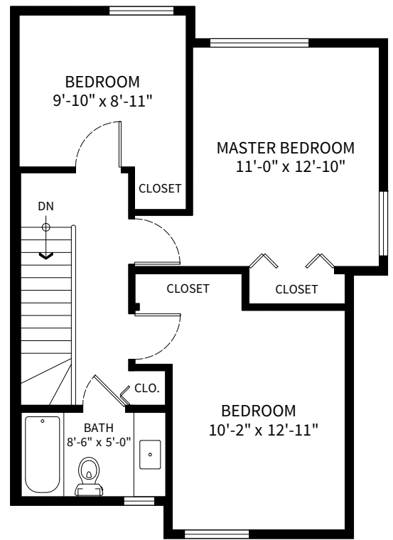
UPPER FLOOR PLAN Ceiling Height: 8'-0"
