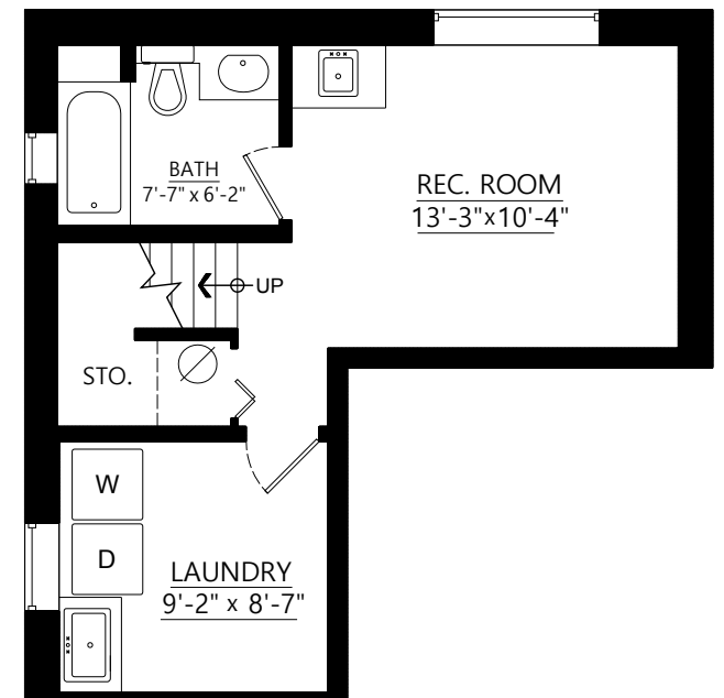
Lower Floor Plan Floor Area: 414 sq.ft.
