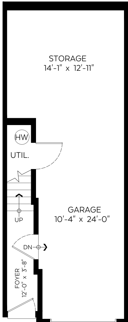
Entry Floor Plan
