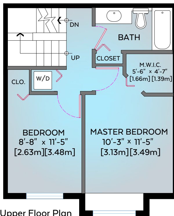
Upper Floor Plan Floor Area: 458 sq.ft. Floor Area: 42.55 sq.m.
