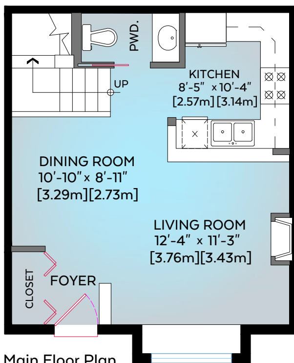
Main Floor Plan Floor Area: 458 sq.ft. Floor Area: 42.55 sq.m.
