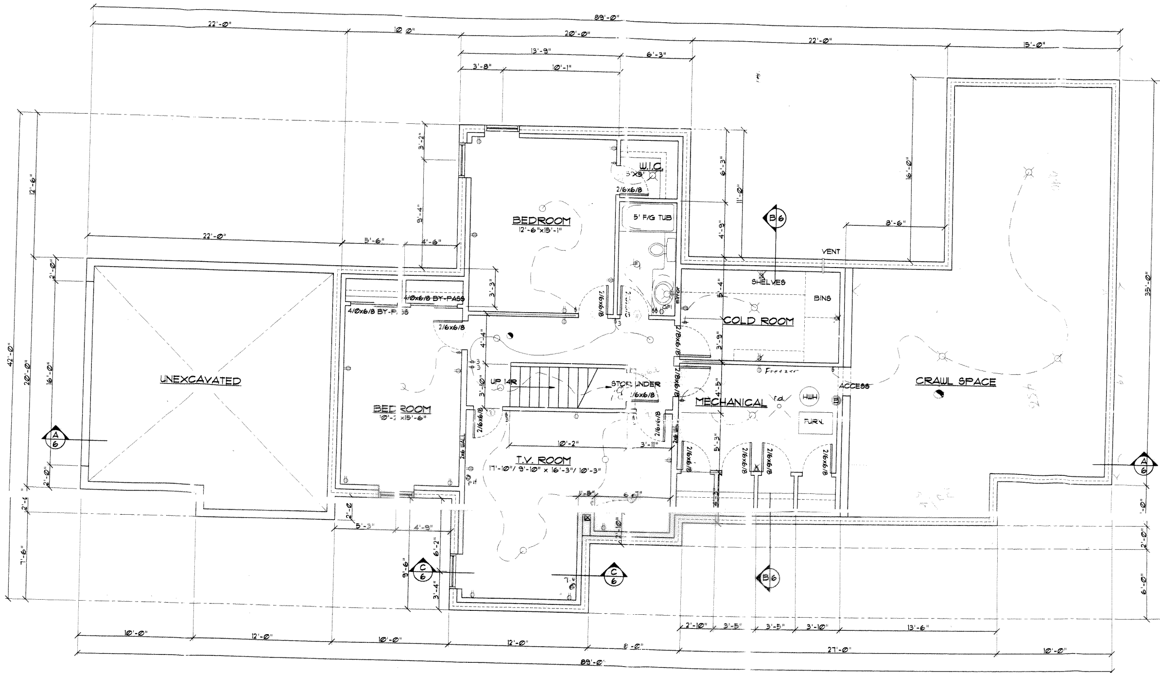
BASEMENT FLOOR PLAN SCALE: 1/4" = 1'-0"
