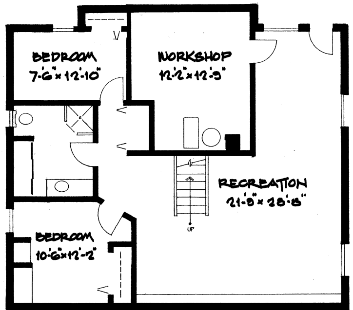
LOWER FLOOR
