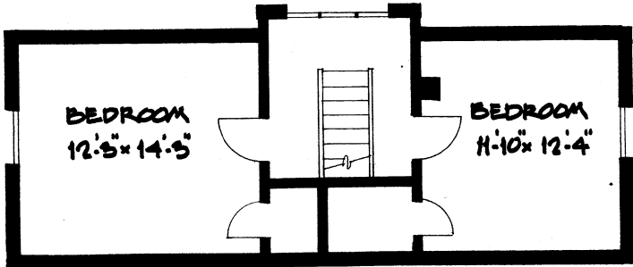
UPPER FLOOR
