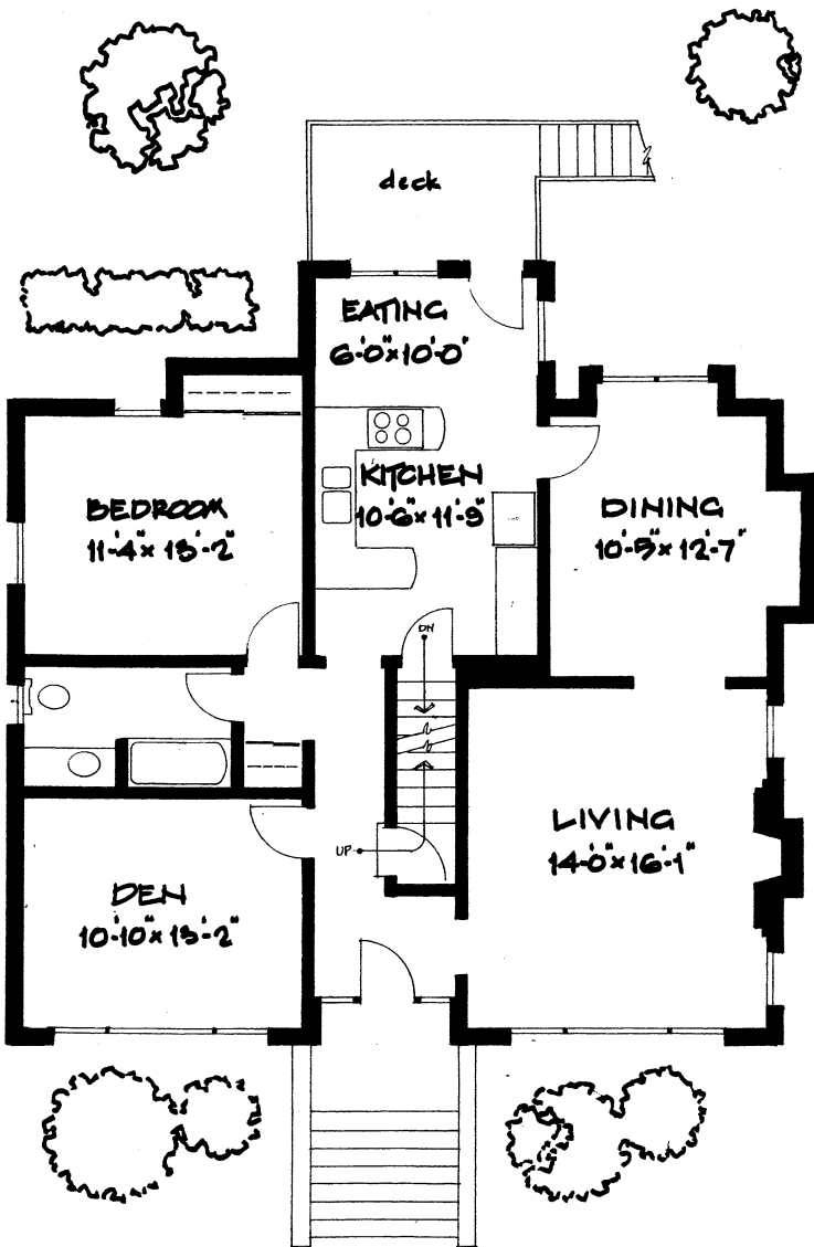
LOWER FLOOR
