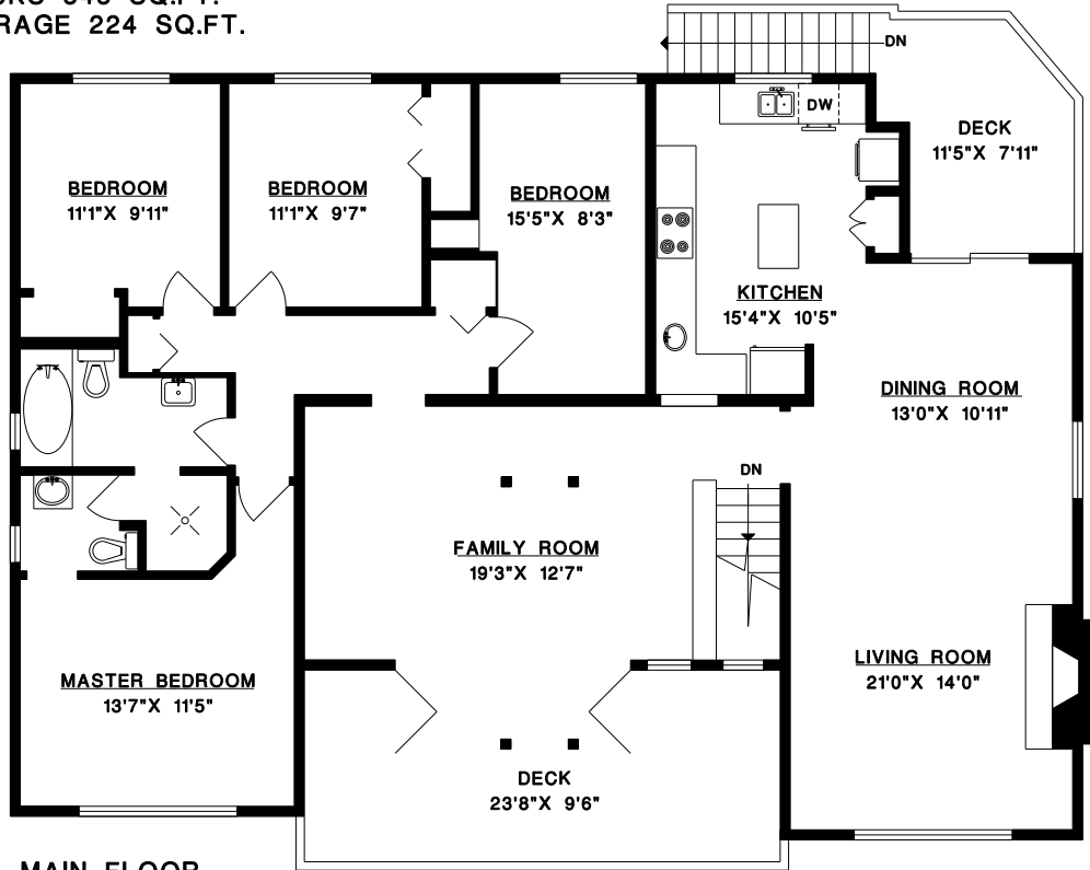
MAIN FLOOR
