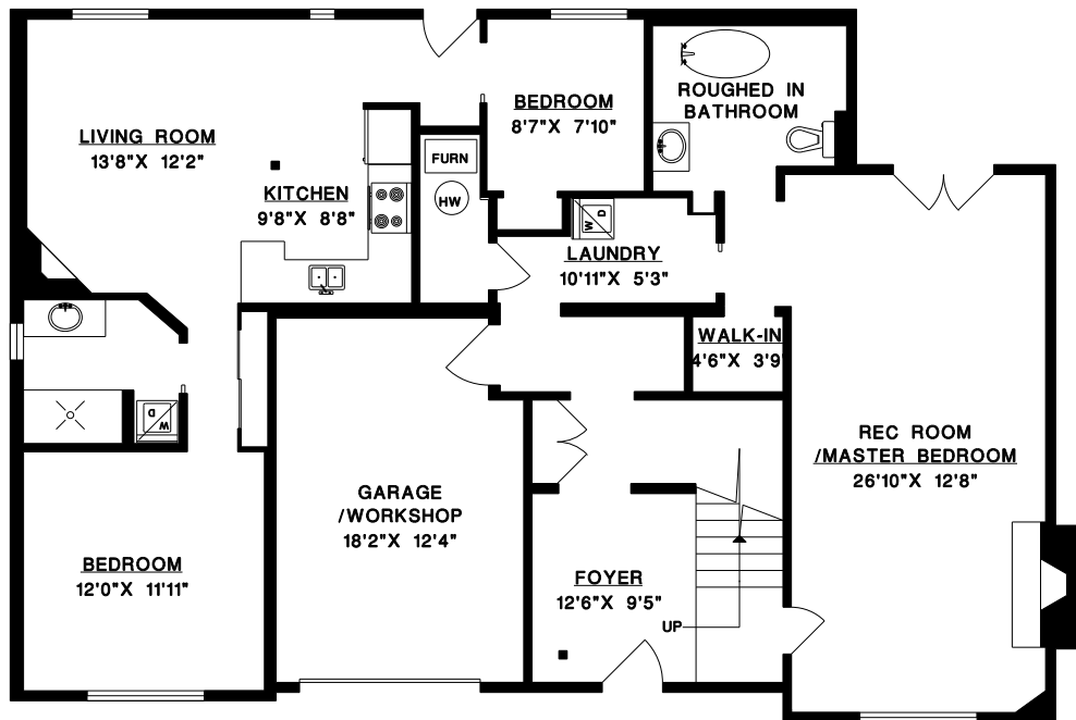
LOWER FLOOR
