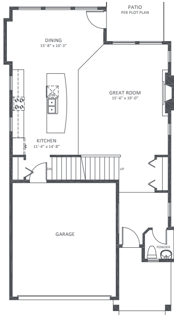
MAIN FLOOR - ELEVATION B Living 930 sq.ft
