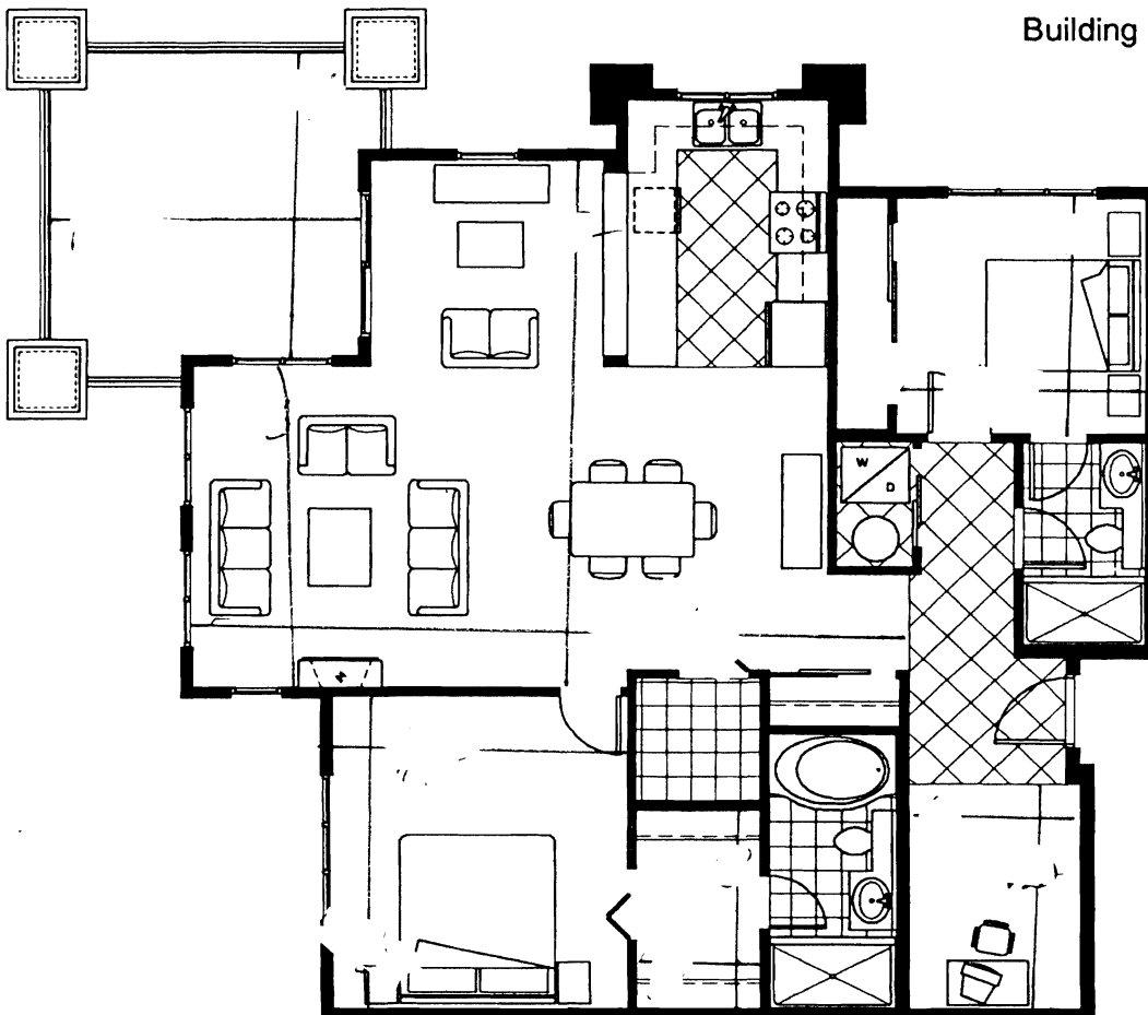
Building D
