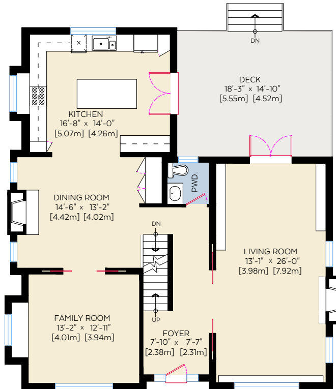
Main Floor Plan Floor Area: 1,312 sq.ft./121.89 sq.m.
