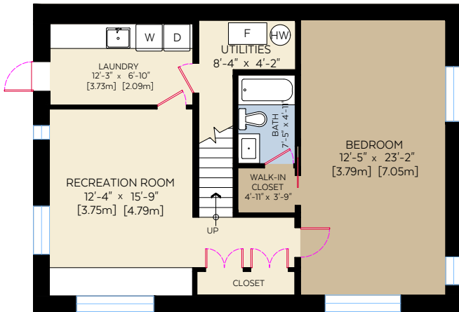
Lower Floor Plan Floor Area: 954 sq.ft./88.63 sq.m.
