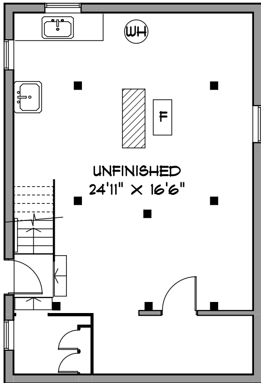
LOWER LEVEL 468 SQ. FT.
