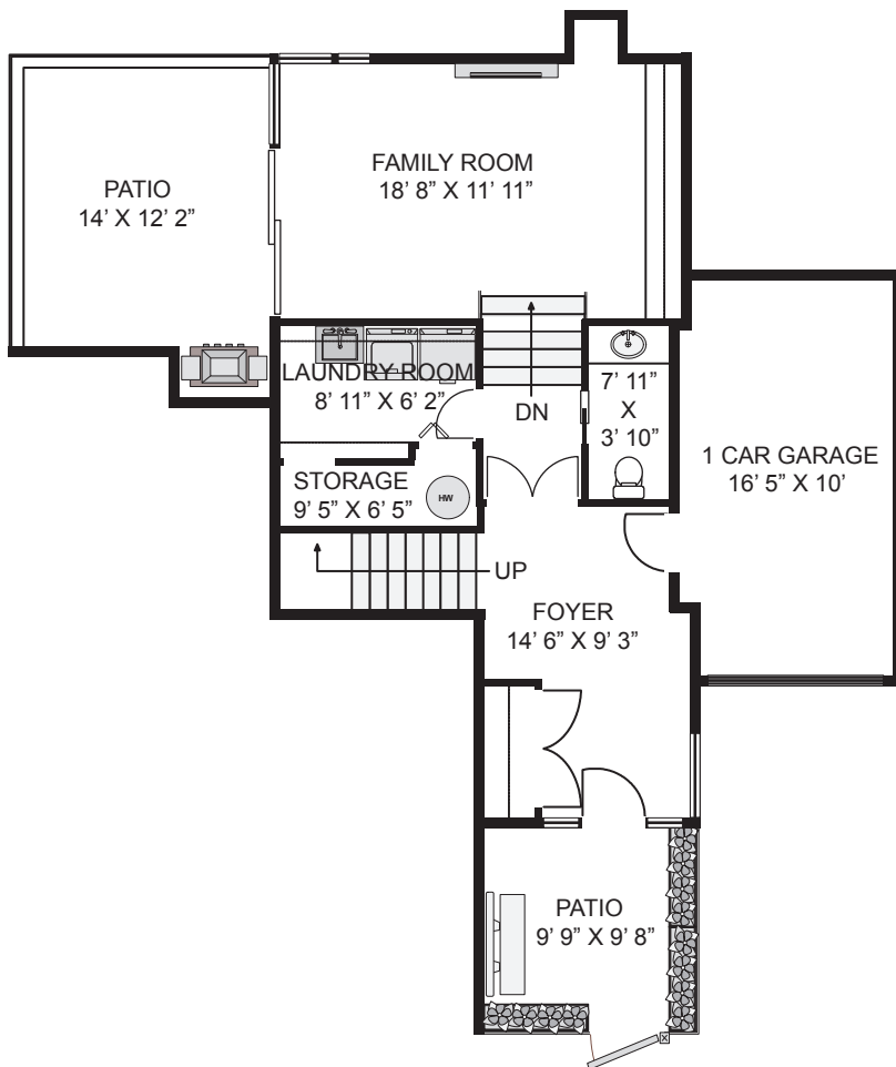
MAIN FLOOR
