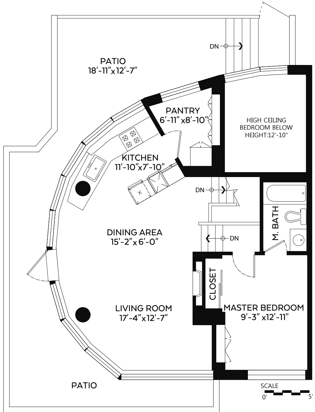
Main Floor Plan Floor Area: 790 sq.ft.
