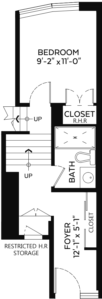
Lower Floor Plan Floor Area: 353 sq.ft.
