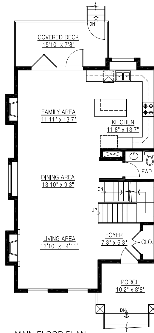
MAIN FLOOR PLAN FLOOR AREA: 915 sq.ft.
