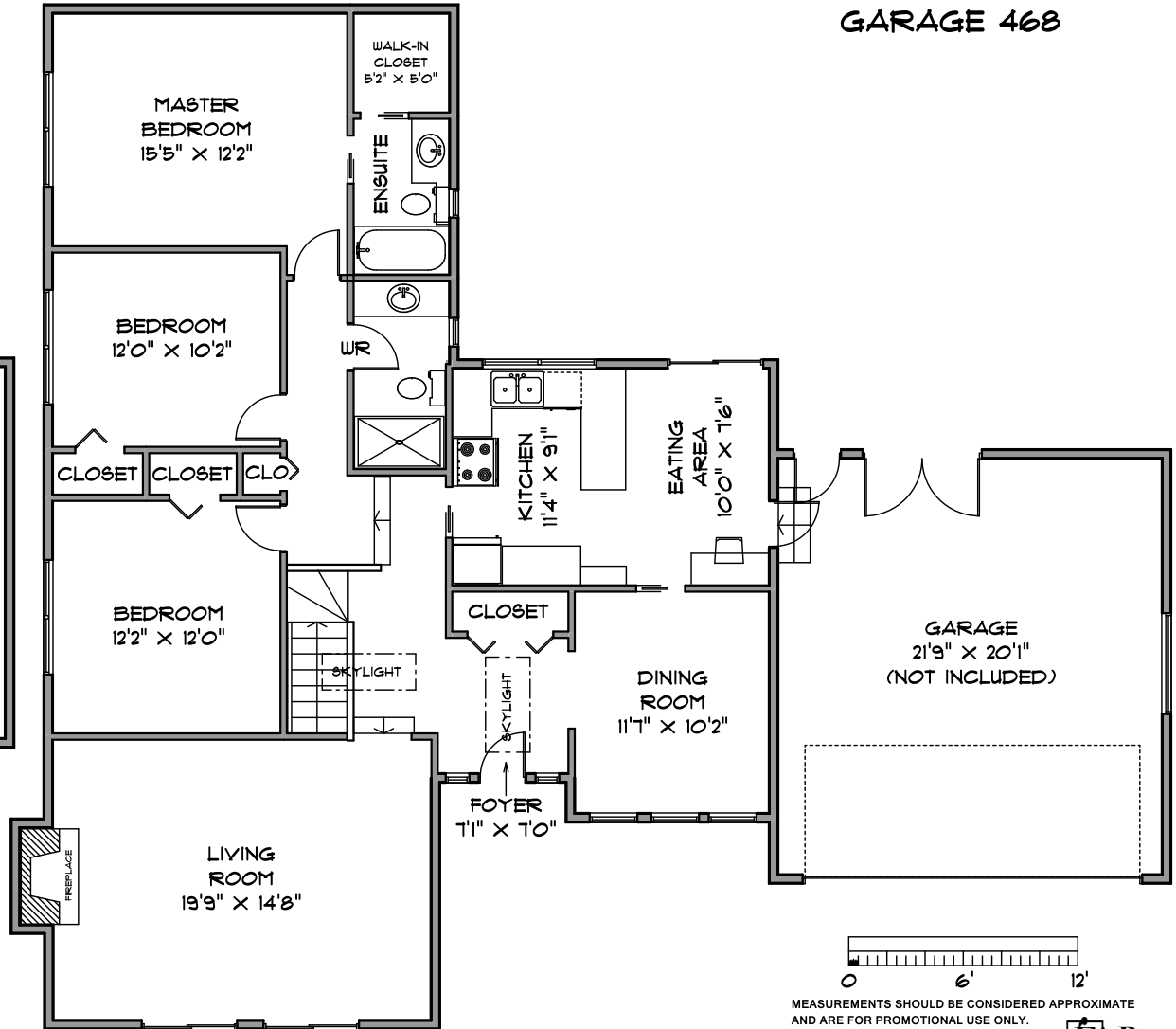
MAIN LEVEL 1560 SQ. FT.
