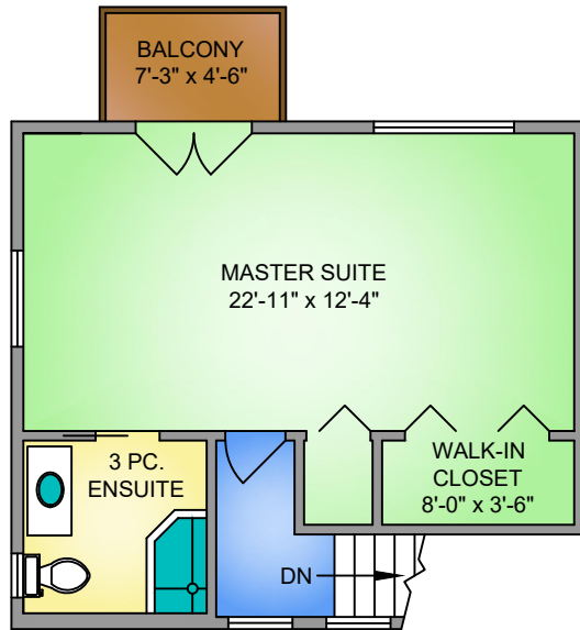
UPPER FLOOR 476 SQ. FT. 8'-0" CEILING HEIGHT
