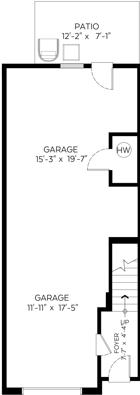
Lower(Entry) Floor Plan
