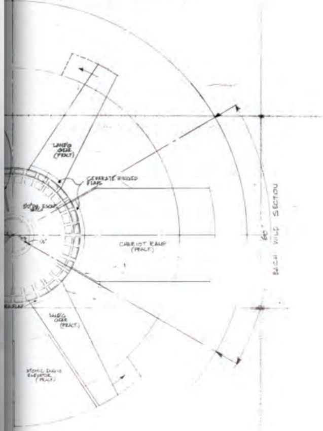
REFLECTED - BOTTOM PLAN SCALE 1/8" = 1'-0"
