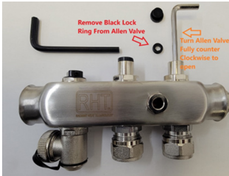
Supply Manifold
