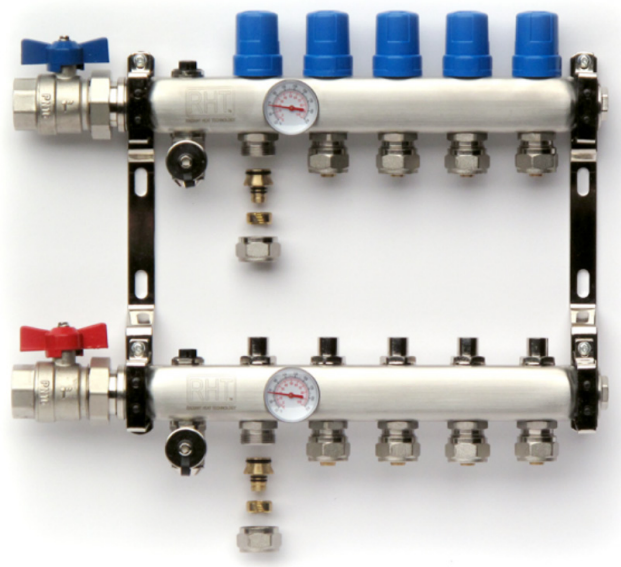
Turn blue valves by hand counterclockwise to open
