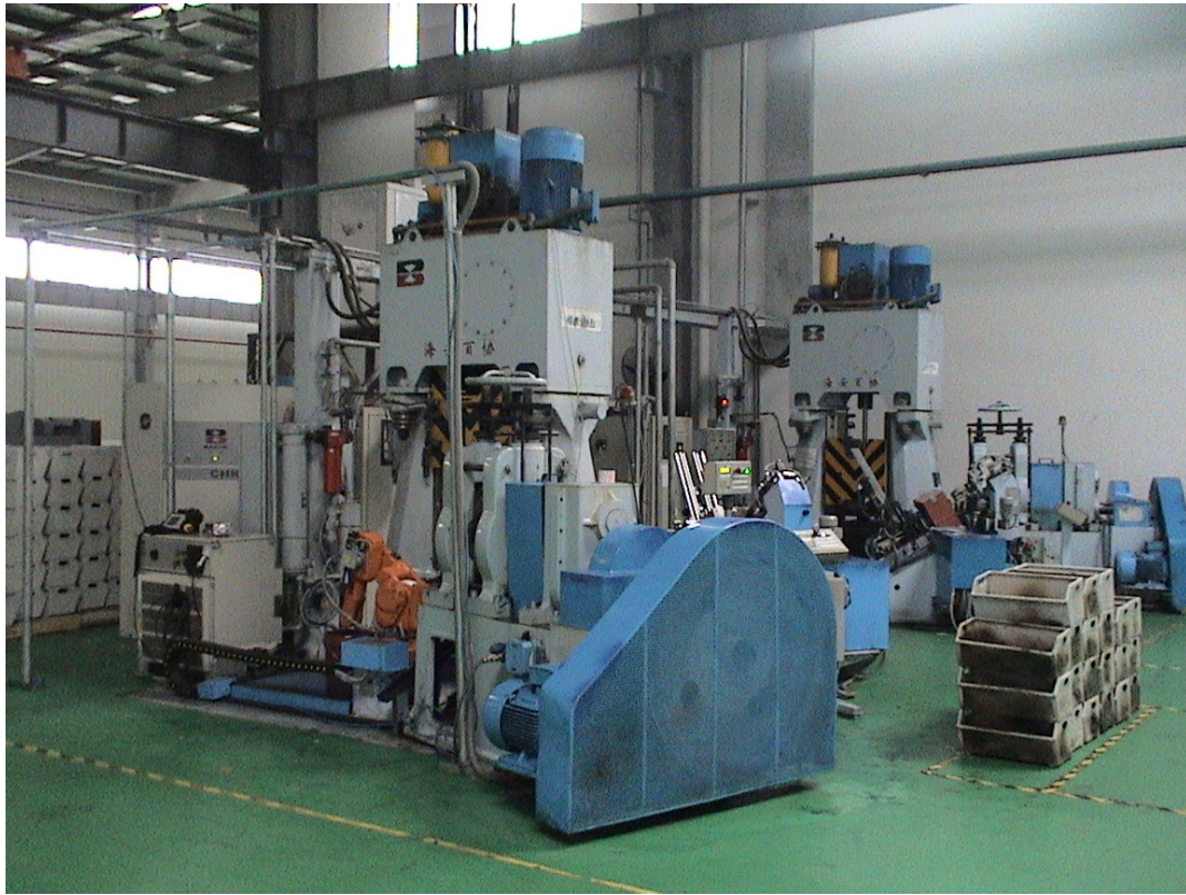
These are two automatic forging lines which are invested by an American in Suzhou, China. They use these two forging lines to produce tablewares.
