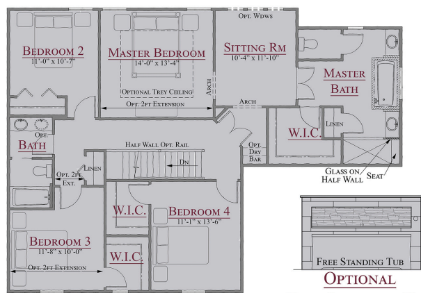
OPT. SECOND FLOOR PLAN EXECUTIVE MASTER SUITE (ADDS 84 S.F.)
