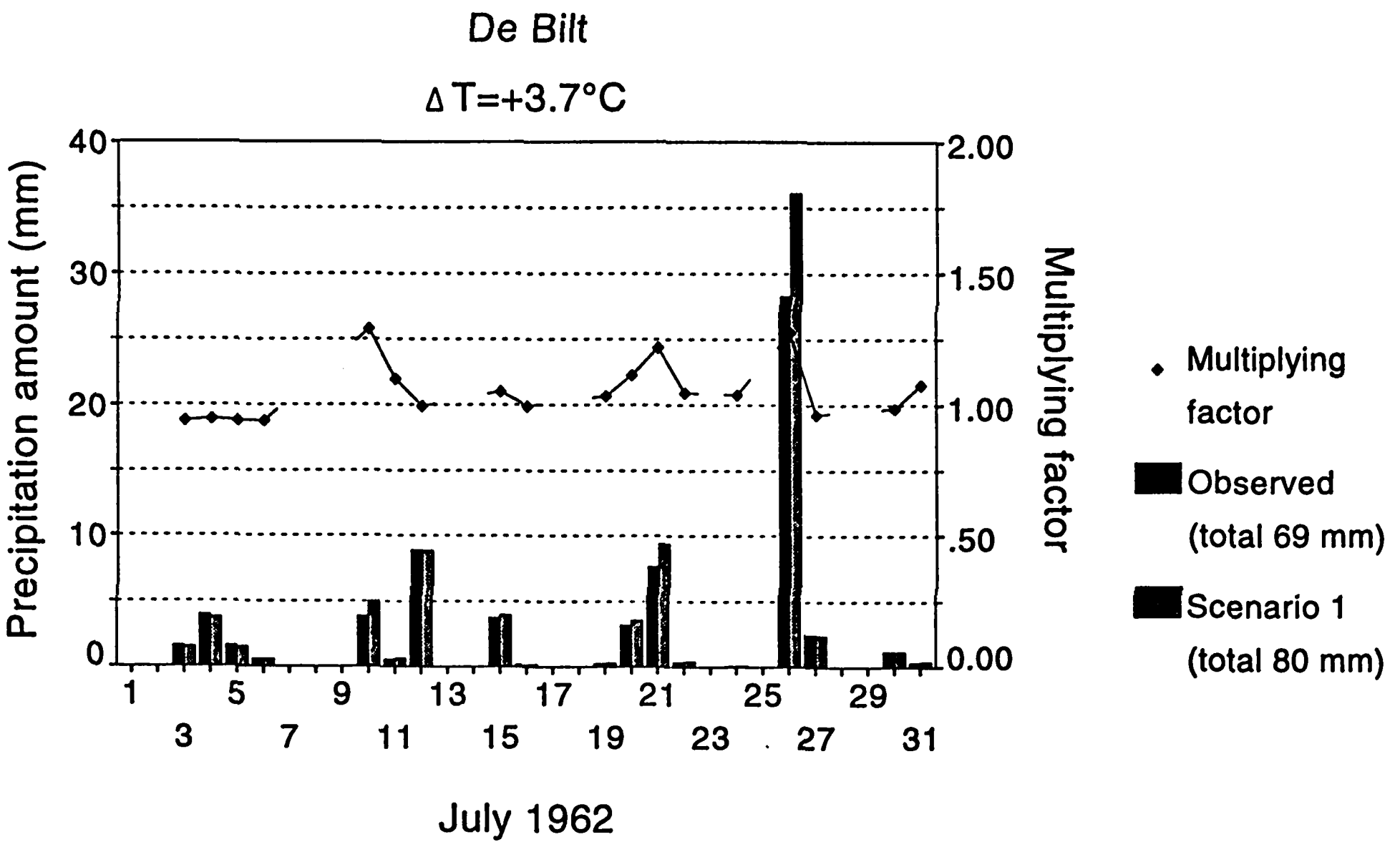
Figure 4. Precipitation amounts in the observed and transformed July 1962 month at De Bilt for Scenario 1. The solid squares represent the multiplying factors.
