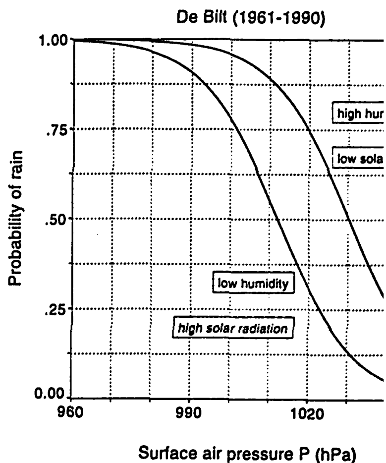
Figure 3. Fitted logistic regression relation for the probability of rain at De Bilt (1961-1990).
