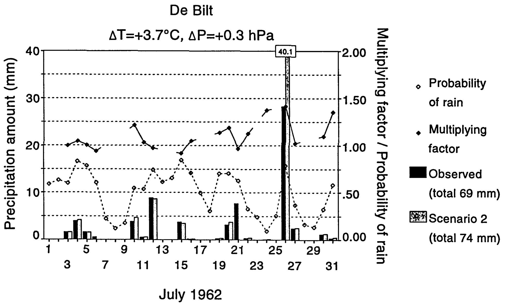
Figure 5. Precipitation amounts in the observed and transformed July 1962 month at De Bilt for Scenario 2. The solid squares represent the multiplying factors and the open squares the probabilities of rain.
