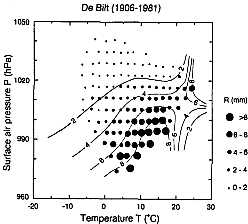
Figure 2. Mean precipitation amounts R (dots) at surface air temperature T class intervals of 2^{\circ}\text{C} and surface air pressure P class intervals of 6 hPa for wet days at De Bilt (1906-1981). The isolines represent the theoretical mean amounts from a fitted regression model. After Buishand and Klein Tank (in press).
