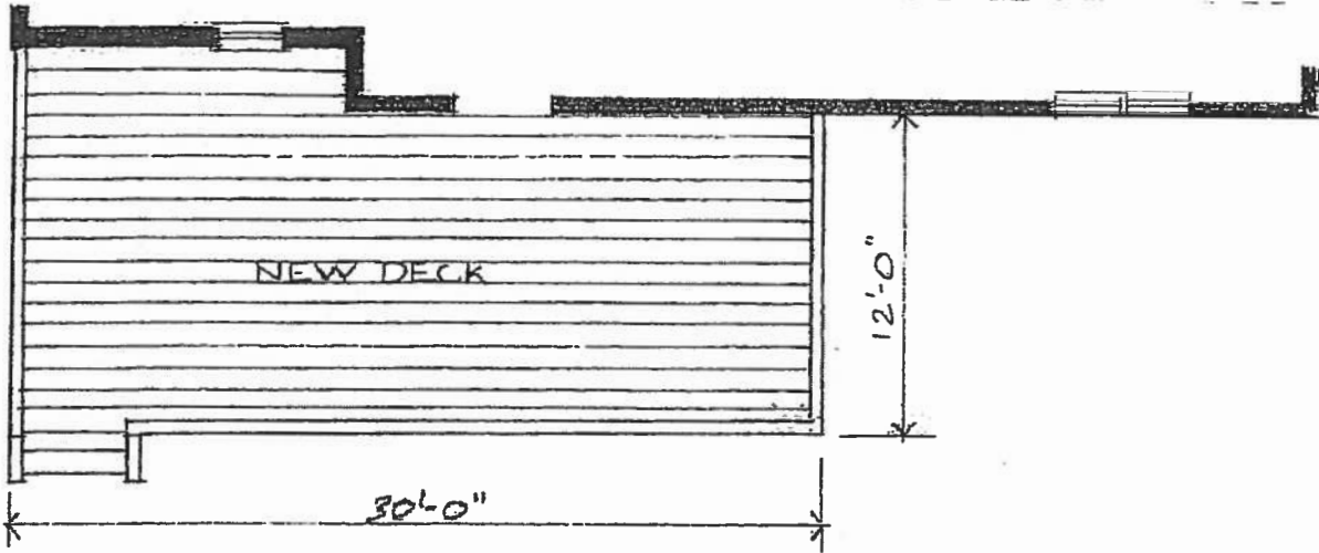
PLAN
