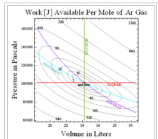
Pressure versus volume plot of available work from a mole of Argon gas relative to ambient, calculated as T_0 times KL divergence.
