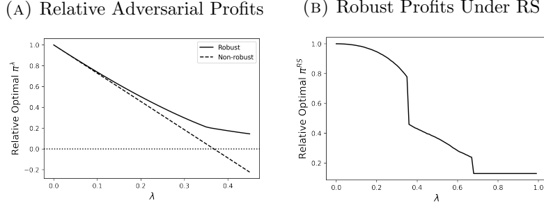
FIGURE 8. Robustness Tests
