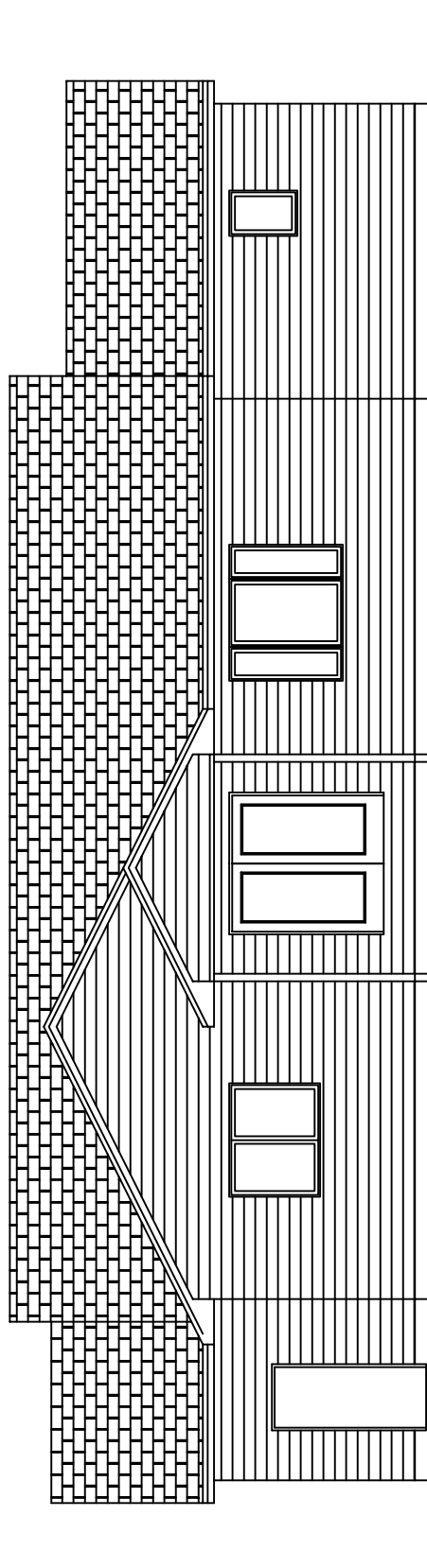
REAR ELEVATION 1/4"=1'-0"
