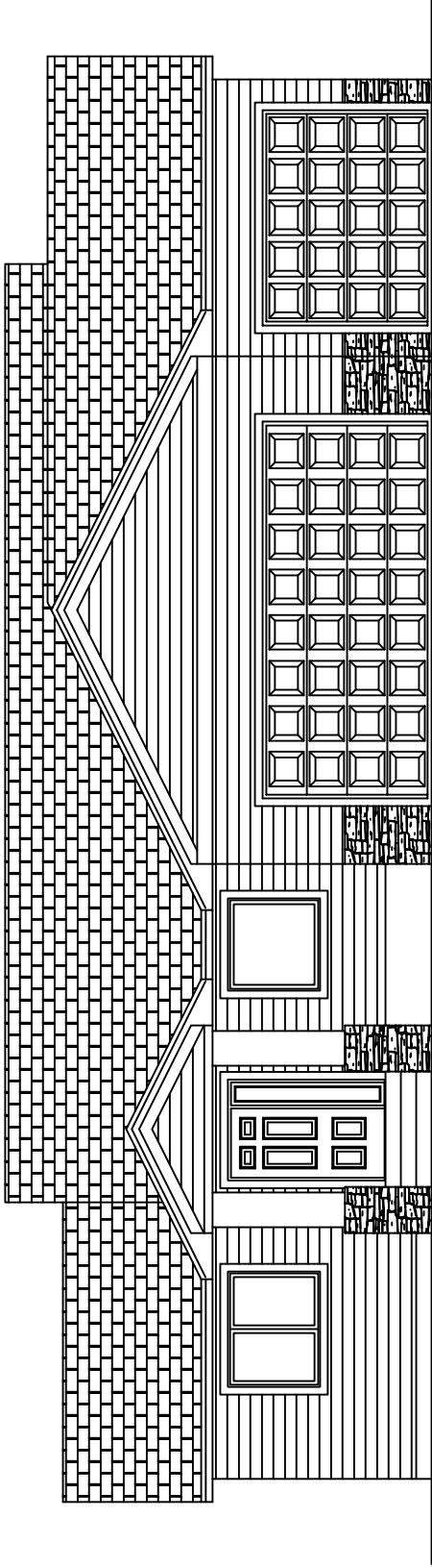
FRONT ELEVATION 1/4"=1'-0"
