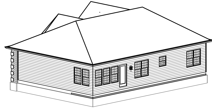
REAR-RIGHT
