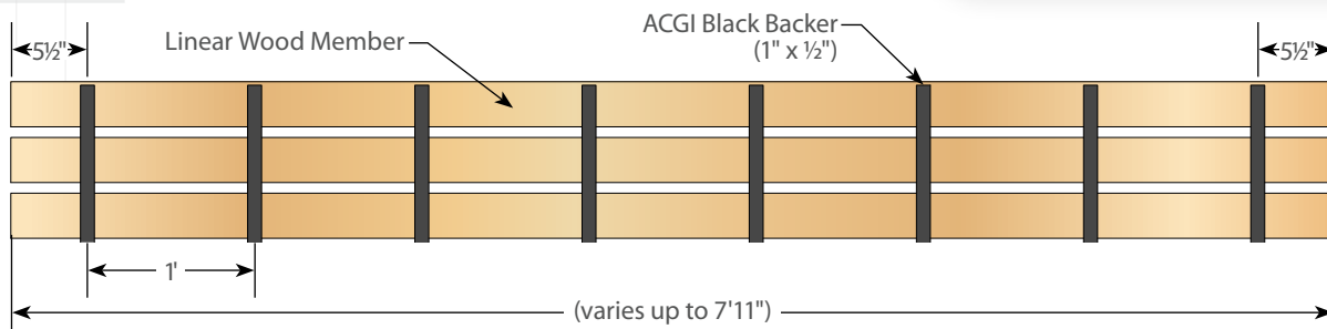
Perimeter Reveal
