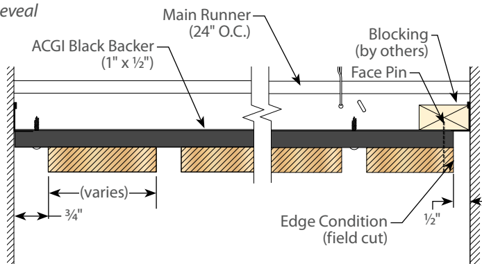
Perimeter Reveal
